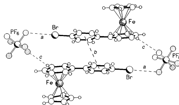
Fig. 2 Back-to-back packing of pairs of [\text{Fe}(\eta^5\text{-C}_5\text{H}_5)(\eta^6\text{-C}_6\text{H}_5\text{C}_6\text{H}_4\text{Br})]^+ cations and their associated [\text{PF}_6]^- anions. The interaction geometries are (a) Br···F 3.20 Å, C–Br···F 178°; (b) centroid ring–centroid ring distance 4.14 Å with a mean interplanar separation of 3.78 Å and (c) C···F 3.43, H···F 2.74 Å and C–H···F 132°
