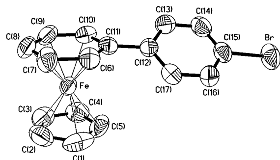
Fig. 1 Molecular structure of the cation [\text{Fe}(\eta^5\text{-C}_5\text{H}_5)(\eta^6\text{-C}_6\text{H}_5\text{C}_6\text{H}_4\text{Br})]^+
